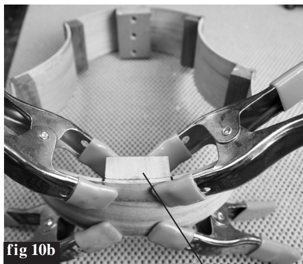
tail block
